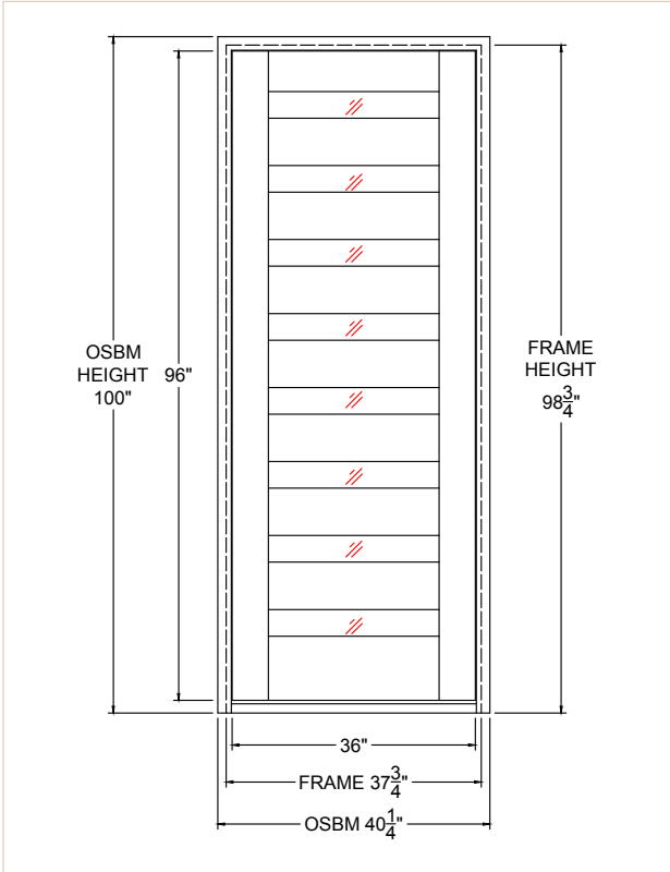
Dimensions In Inches · 3080
